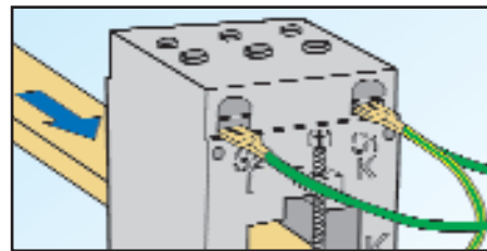
WITH FAST-ON (6,3 mm)
