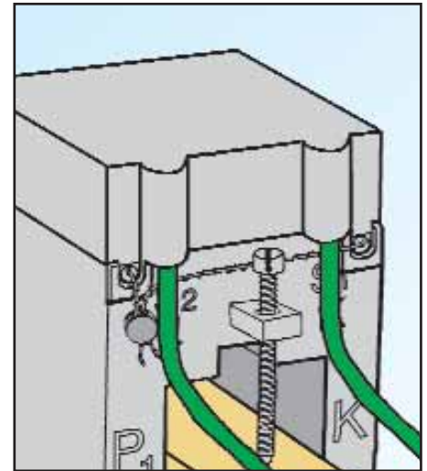
FIXING OF TERMINALS COVER AND LEAD SEAL
