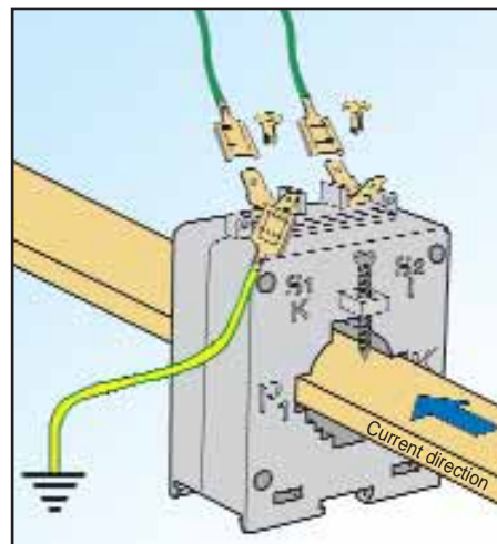
WITH FAST-ON (6,3 mm)
