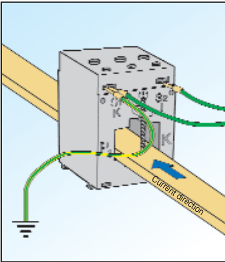
WITH METAL POINT CABLE TERMINAL
