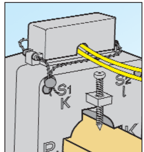
FIXING OF TERMINALS COVER AND LEAD SEAL
