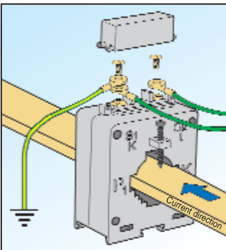
WITH METAL FORK CABLE TERMINAL
